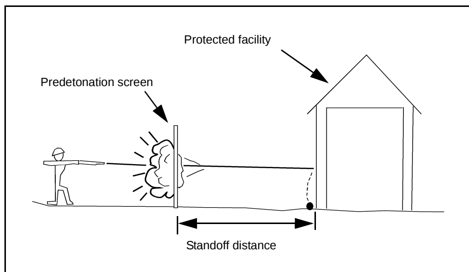
Figure 3-10. Predetonation Screen
